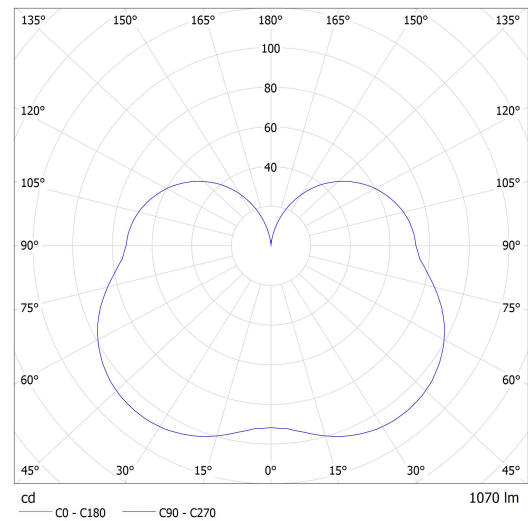
Luminaire: Lucis ZL1.IC.K2.150.X IZAR C LED Lamps: 1 x LED 103/73-G5
