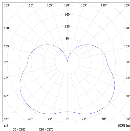
Luminaire: Lucis ZL1.IC.K1.250.X IZAR C LED Lamps: 1 x LED D180-G5
