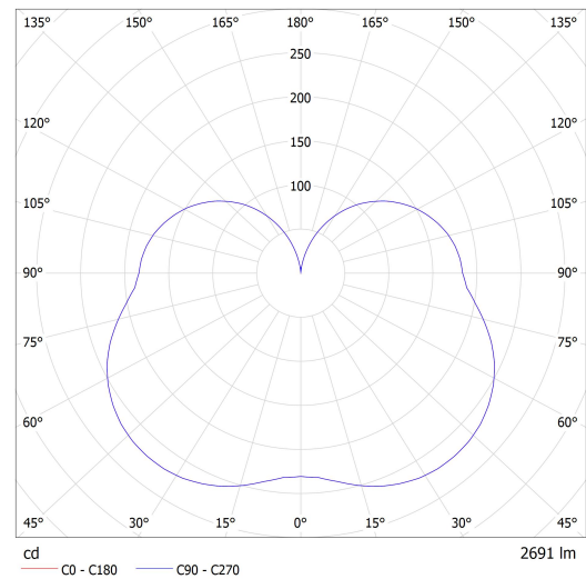
Luminaire: Lucis ZL1.IC.K1.330.X IZAR C LED Lamps: 1 x LED D180-G5
