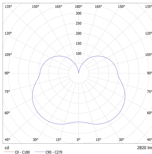
Luminaire: Lucis ZL1.IC.K2.330.X IZAR C LED Lamps: 1 x LED D180-G5
