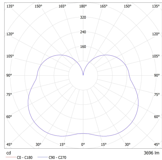
Luminaire: Lucis ZL4.IC.K1.440.X IZAR C LED Lamps: 1 x LED 252/160-G5
