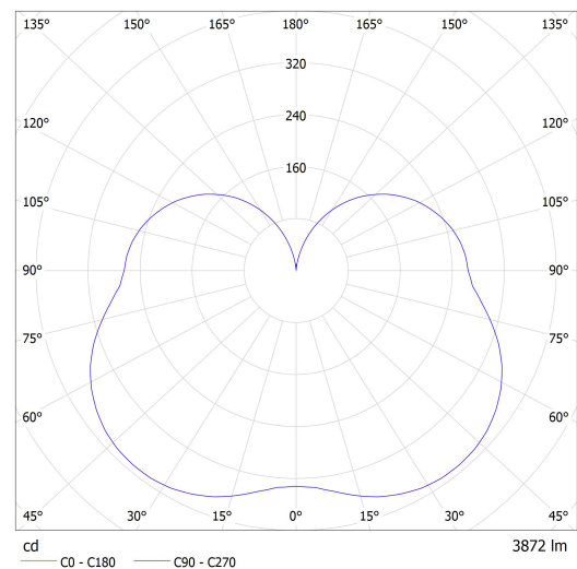
Lucis ZL4.IC.K2.440.X IZAR C LED / LDC (Polar)
