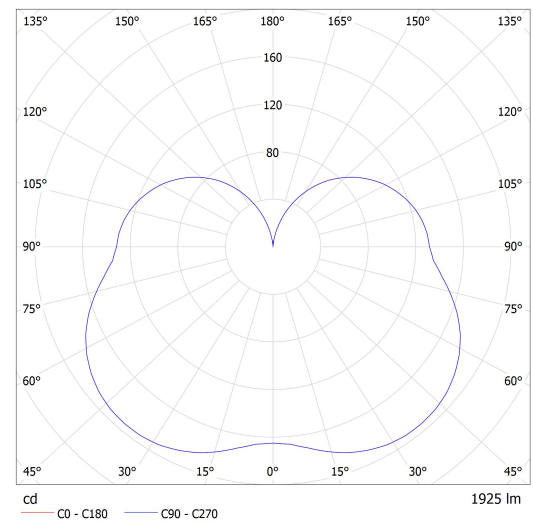
Lucis IC.K1.250.X IZAR C LED / LDC (Polar)
