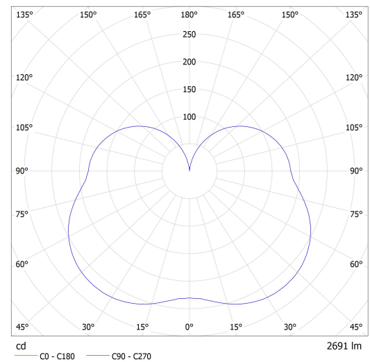
Lucis IC.K1.330.X IZAR C LED / LDC (Polar)
