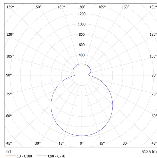
Lucis ZL3.K1.O60 FORUM LED / LDC (Polar)
