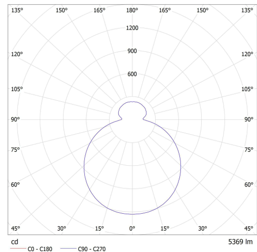
Lucis ZL3.K2.O60 FORUM LED / LDC (Polar)
