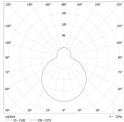
Luminaire S43.114.Z500 ZERO / LDC (Polar)
