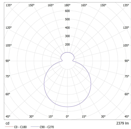
Lucis S34.K3.Z415 ZERO LED / LDC (Polar)
