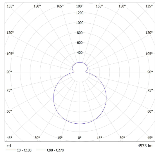
Luminaire: Lucis S43.K1.Z500 ZERO LED / LDC (Polar)
