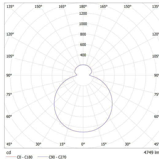
Luminaire: Lucis S43.K2.Z500 ZERO LED / LDC (Polar)
