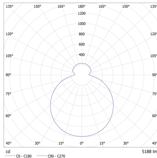
Lucis S46.K1.Z600 ZERO LED / LDC (Polar)
