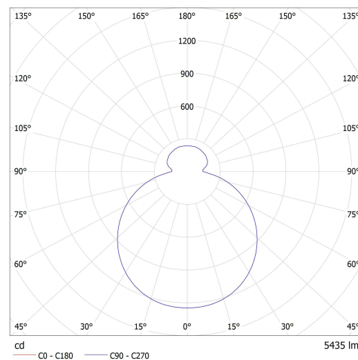
Lucis S46.K2.Z600 ZERO LED / LDC (Polar)
