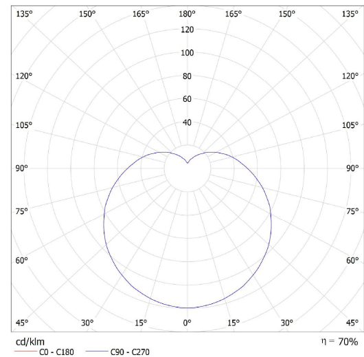
Lucis S29.112.JS33 LEDA / LDC (Polar)
