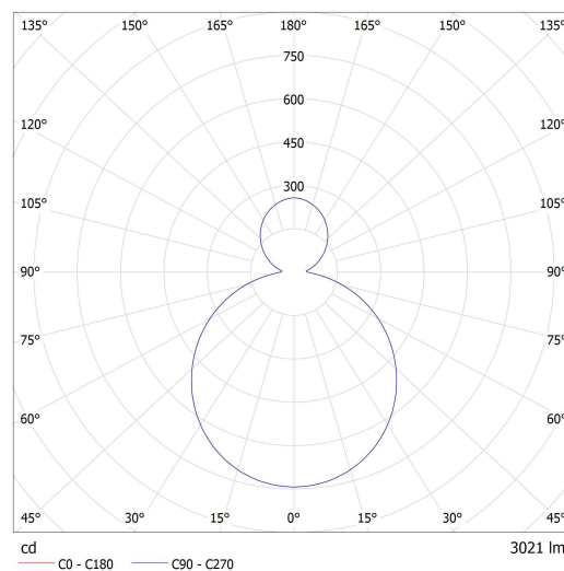
Lucis S34.K1.R550 RONDO LED / LDC (Polar)
