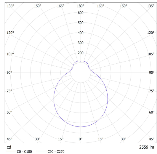
Luminaire: Lucis S37.L1.JS41 LEDA LED Lamps: 1 x LED G6
