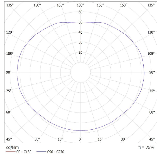
Lucis S00.11.115.X ALFA / LDC (Polar)
