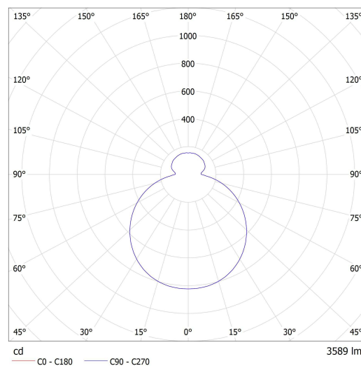
Lucis S34.K2.O42 FORUM LED / LDC (Polar)
