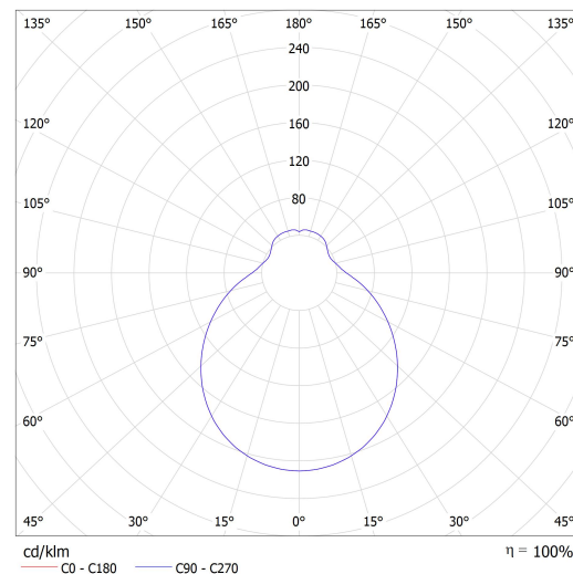
Luminaire: Lucis S24.L1.AN2 ANANKE LED Lamps: 1 x LED G6
