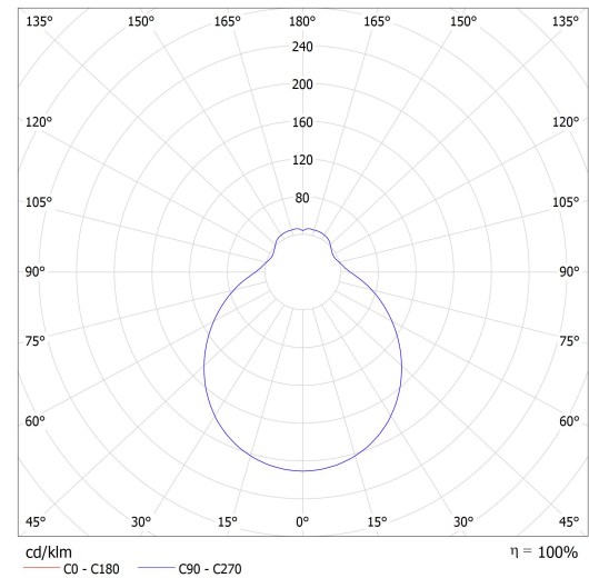
Luminaire: Lucis S24.L2.AN2 ANANKE LED Lamps: 1 x LED G6
