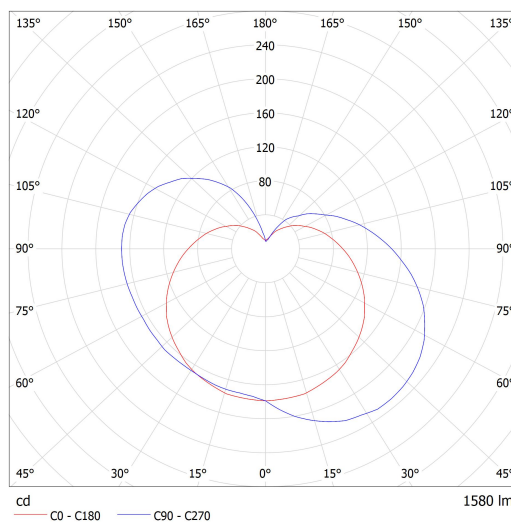
Luminaire: Lucis CS32.L1 SINOPE LED Lamps: 1 x LED G6
