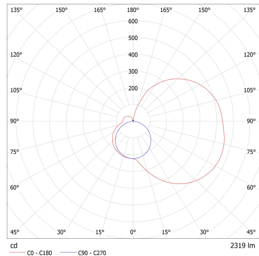
Luminaire: Lucis I1.L2.600.X IZAR I LED Lamps: 1 x LED G6
