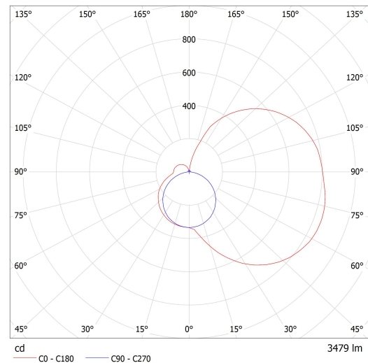
Luminaire: Lucis I1.L2.900.X IZAR I LED Lamps: 1 x LED G6
