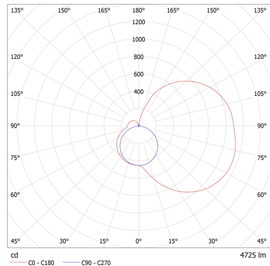
Luminaire: Lucis I1.L1.1200.X IZAR I LED Lamps: 1 x LED G6
