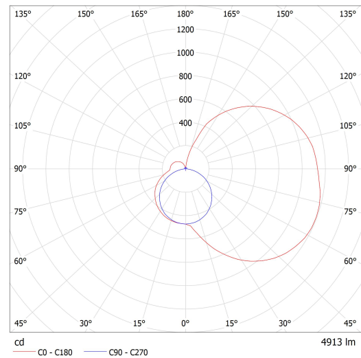
Luminaire: Lucis I1.L2.1200.X IZAR I LED Lamps: 1 x LED G6
