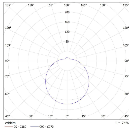
Lucis S56.113.CA6 CHARON PMMA / LDC (Polar)
