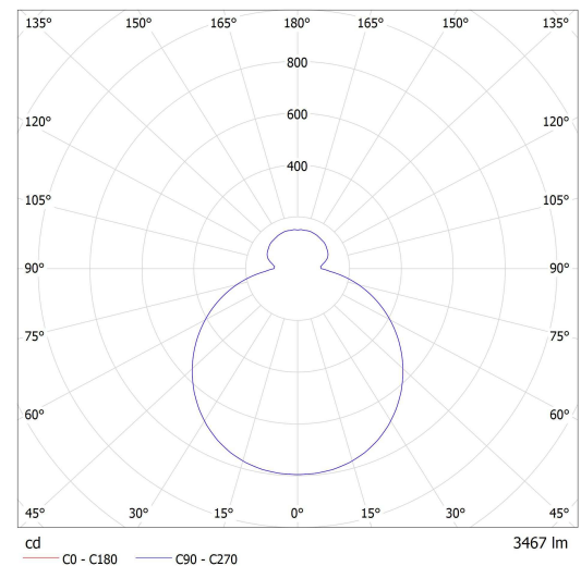
Lucis ZL3.K1.Z415 ZERO LED / LDC (Polar)
