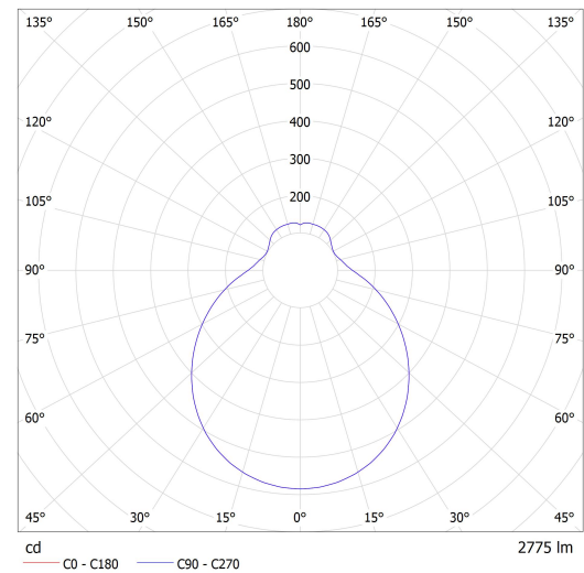
Luminaire: Lucis S37.L1.T14 CHARON LED Lamps: 1 x LED G6
