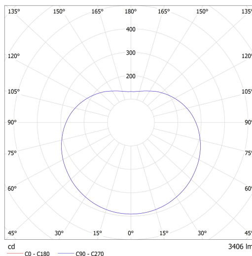
Luminaire: Lucis ZT.P1.400.X POLARIS ZT LED Lamps: 1 x LED G6
