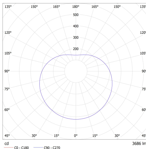
Luminaire: Lucis ZT.P2.400.X POLARIS ZT LED Lamps: 1 x LED G6
