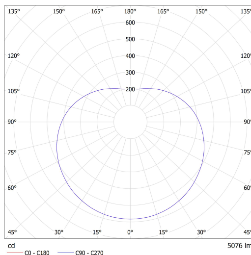
Luminaire: Lucis ZT.P1.500.X POLARIS ZT LED Lamps: 1 x LED G6
