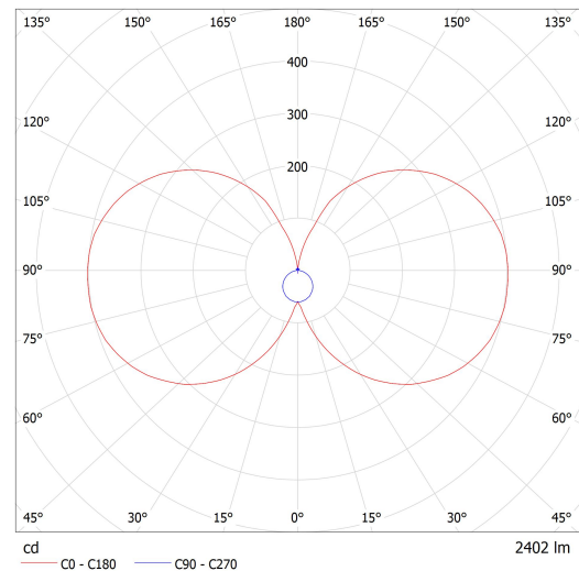
Lucis I2.L1.600.X IZAR II LED / LDC (Polar)
