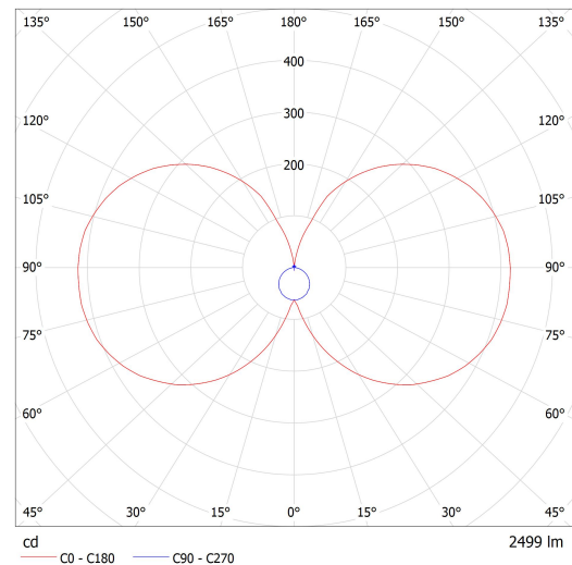
Luminaire: Lucis I2.L2.600.X IZAR II LED Lamps: 1 x LED G6
