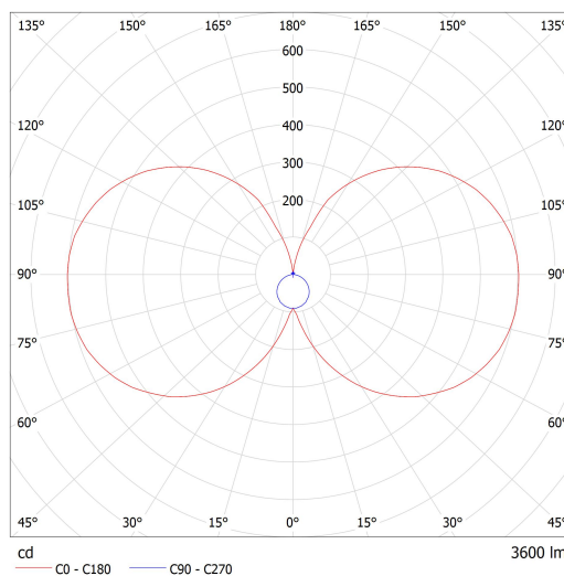
Lucis I2.L1.900.X IZAR II LED / LDC (Polar)
