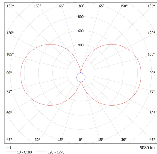
Lucis I2.L1.1200.X IZAR II LED / LDC (Polar)
