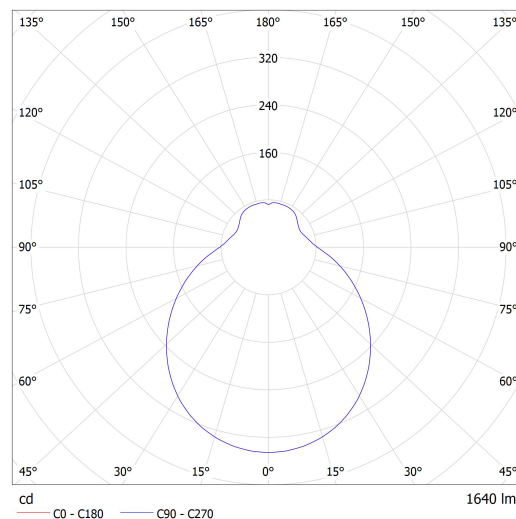
Luminaire: Lucis S29.L3.T135 CHARON LED Lamps: 1 x LED G6
