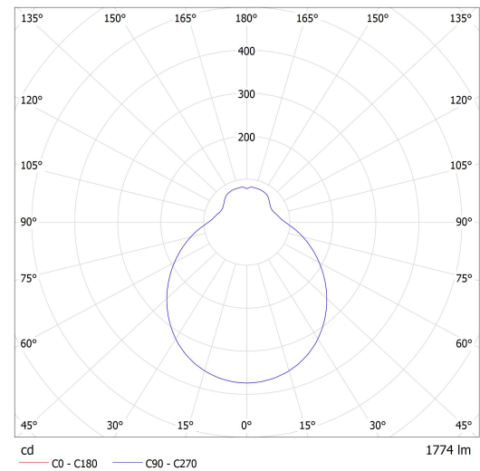
Luminaire: Lucis S29.L4.T135 CHARON LED Lamps: 1 x LED G6
