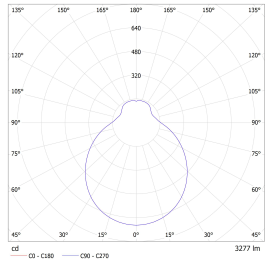
Luminaire: Lucis S43.L3.T15 CHARON LED Lamps: 1 x LED G6
