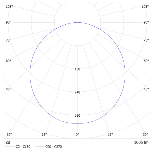
Luminaire: Lucis O.525.K2.X OMNIA LED Lamps: 1 x LED G5
