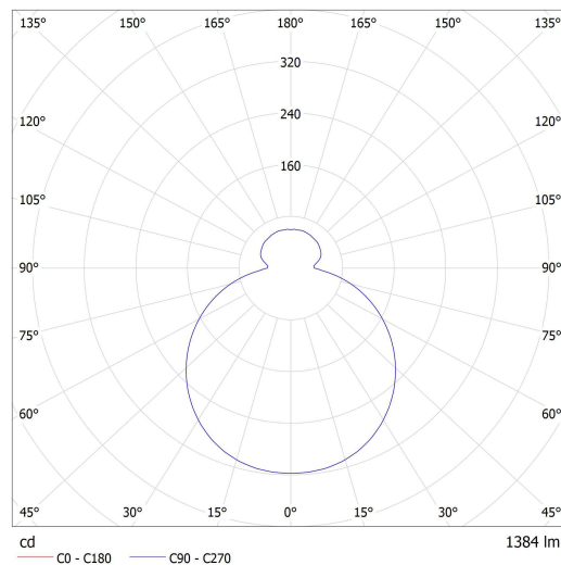
Luminaire: Lucis S29.K4.Z330 ZERO LED Lamps: 1 x LED G5
