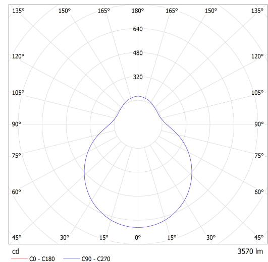
Luminaire: Lucis ZL3.L1.D451.X DAPHNE LED Lamps: 1 x LED G6
