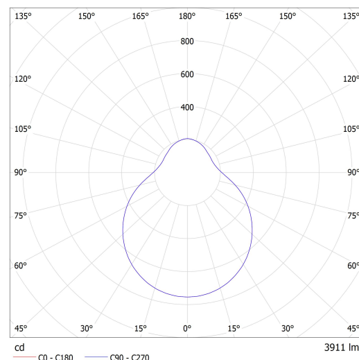
Luminaire: Lucis ZL3.L2.D451.X DAPHNE LED Lamps: 1 x LED G6
