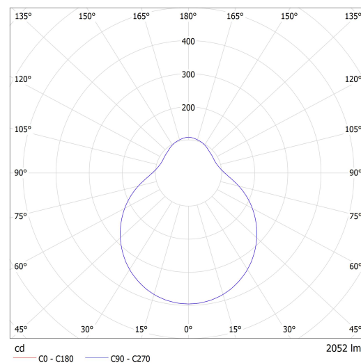
Luminaire: Lucis S24.L2.D350 DAPHNE LED Lamps: 1 x LED G6
