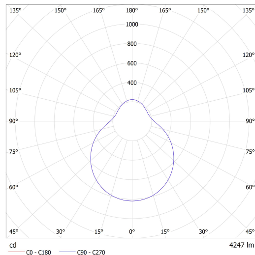
Luminaire: Lucis S43.L1.D550 DAPHNE LED Lamps: 1 x LED G6
