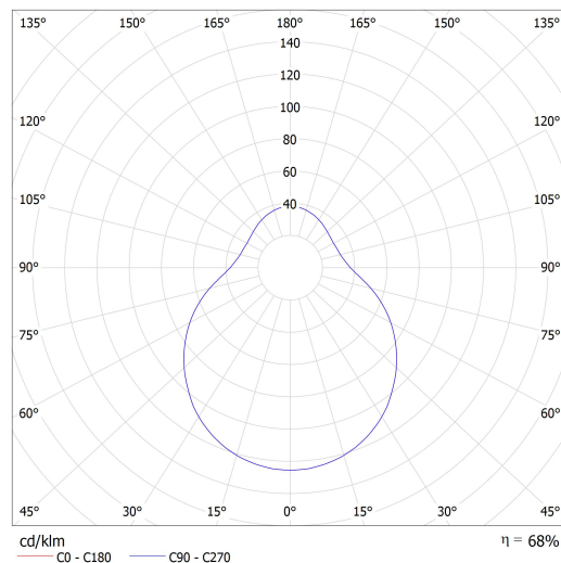
Luminaire: Lucis PS13.12.D350 DAPHNE Lamps: 2 x Osram CL 60W
