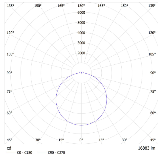
Lucis IB.L2.900.X IZAR B LED / LDC (Polar)
