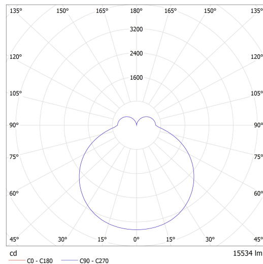
Lucis IB.L1.900M.X IZAR B MAX LED / LDC (Polar)
